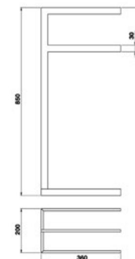
QU 090910 Porta Salviette Free-Standing Towel Rail Porte-Serviette
