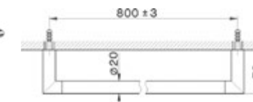
SY 090103 Porta Salviette Towel Rail Porte-Serviette
