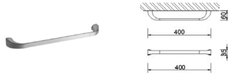
AE 090101 Porta Salviette Towel Rail Porte-Serviette
