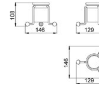
AR 090470 Porta Bicchieri Toothbrush Holder Porte-Verre
