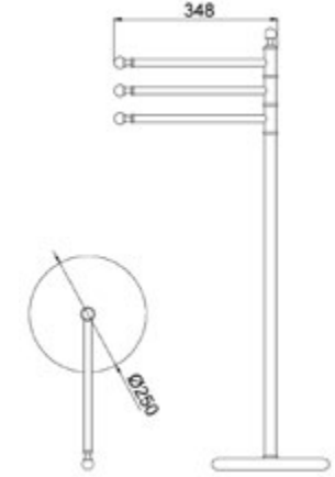
AR 090910 Porta Salviette Free-Standing Towel Rail Porte-Serviette
