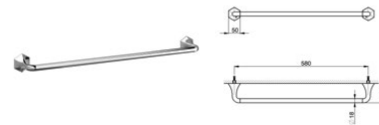
CE 090102 Porta Salviette Towel Rail Porte-Serviette
