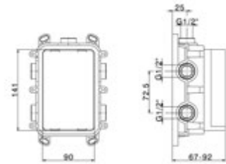
ZA 00B030 Parte Incasso ONE Box ONE Box Concealed Part Partie Encastrée ONE Box
