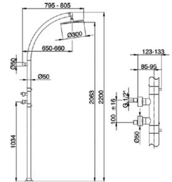
LN C90010 Colonna Doccia Termostatica Thermo Shower Column Colonne de Douche Thermo
