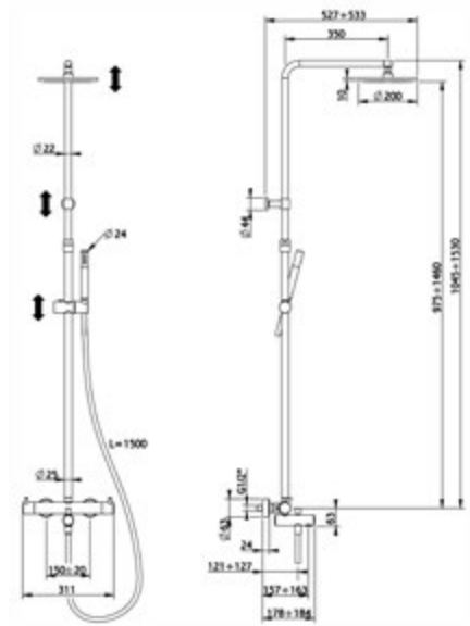
LN C8501D CombiVasca Termostatico Thermo CombiBath CombiBain Thermo
