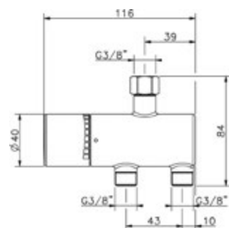
TX T83010 Termostatico Sottolavabo Underbasin Thermo Thermo Sous Lavabo
