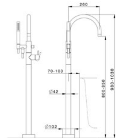
LN 014200 Parte Esterna Monocomando Vasca Free-Standing Free-Standing Bath/S. Mixer Exposed Part Partie Apparente Mitigeur Bain/D. Free-Standing
