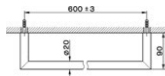
SY 090102 Porta Salviette Towel Rail Porte-Serviette
