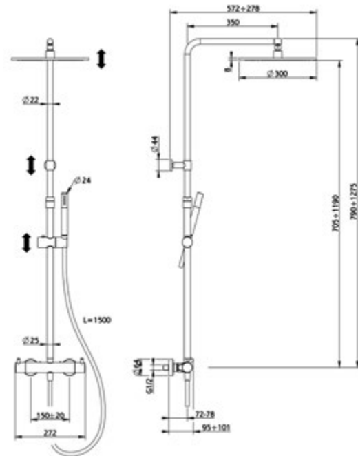
LN C8401D CombiDoccia Termostatico Thermo CombiShower CombiDouche Thermo
