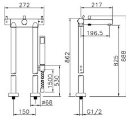
LN T39010 Completo Termostatico Vasca Free-Standing Free-Standing Bath/S. Thermo Set Ensemble Thermo Bain/D. Free-Standing
