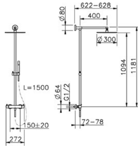
LN C7801N CombiDoccia Termostatico Thermo CombiShower CombiDouche Thermo
