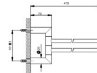
SY 090210 Porta Salviette Towel Rail Porte-Serviette
